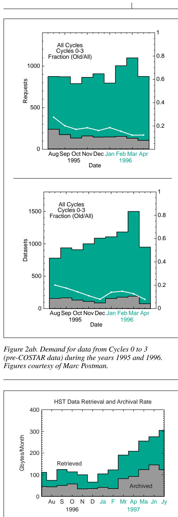
Figure 3. Demand for all HST data during the time between July 1996 and July 1997.
